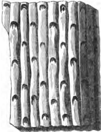
SIGILLARIA PACHYDERMA. (One-fourth nat. size.)
